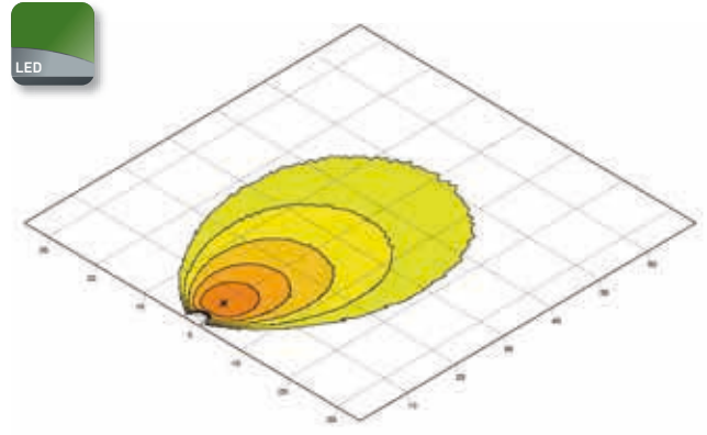
Oval 100 LED | Close-range illumination Page 59
