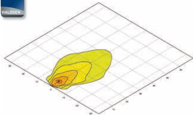
Picador | Close-range illumination Page 76
