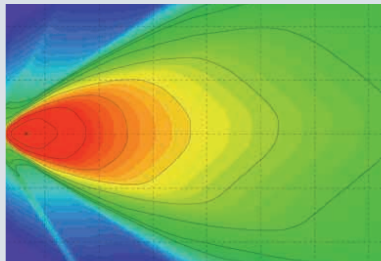
Computer simulation of the superimposed light produced by 2 x Oval 90 LED worklights shows how a harmonious overall pattern is produced.
