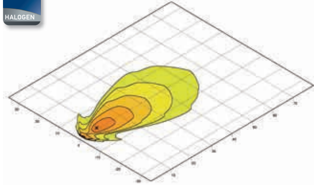
Module 70, H3 | Close-range illumination Page 81
