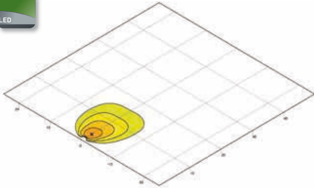
Flat Beam 500 | Close-range illumination Page 68
