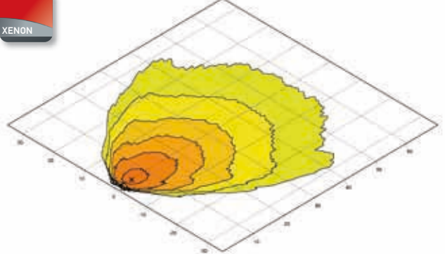
Oval 100 X-PowerPack | Close-range illumination Page 70
