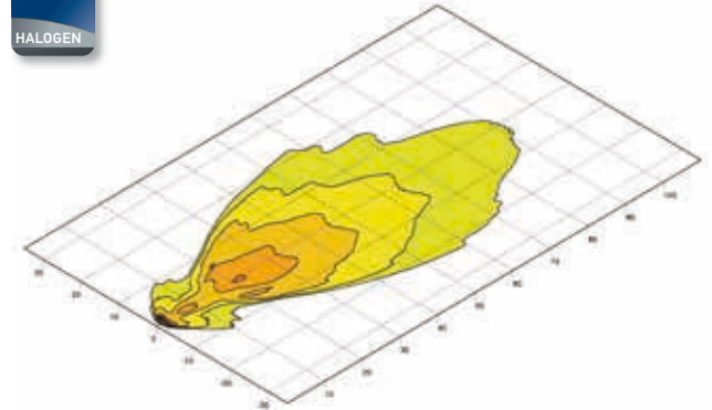
Oval 100 Double Beam | Close-range illumination Page 82
