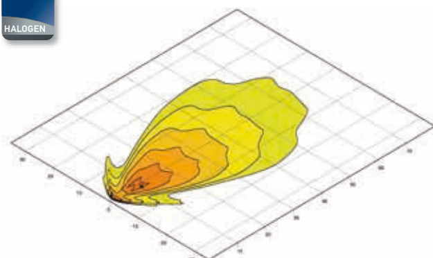
Modul 70, H9 | Close-range illumination Page 80
