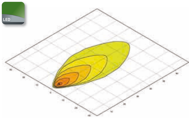
Power Beam 1500 | Close-range illumination Page 60
