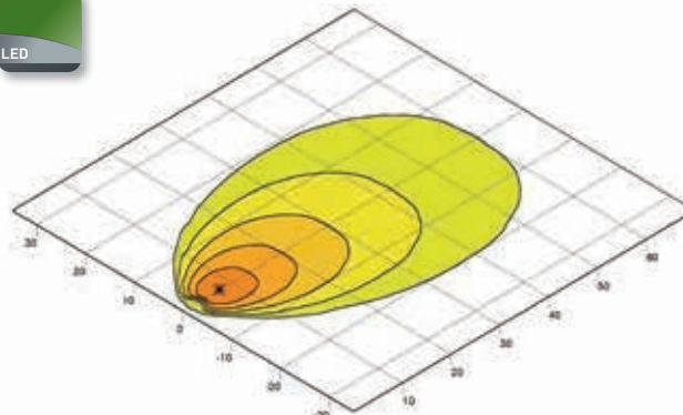
Power Beam 1800 | Close-range illumination Page 57
