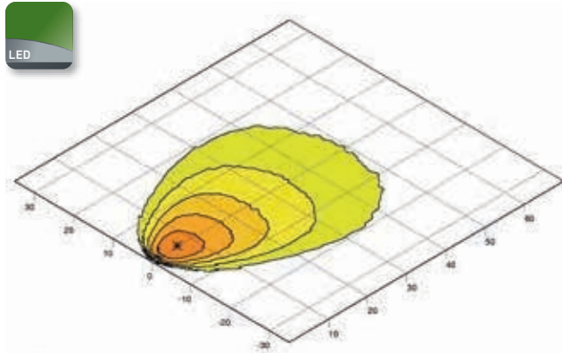
Modul 70 LED Gen. IV | Close-range illumination Page 58
