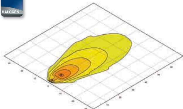
Double Beam | Close-range illumination Page 78
