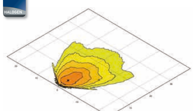
Oval 100 FL | Close-range illumination Page 84
