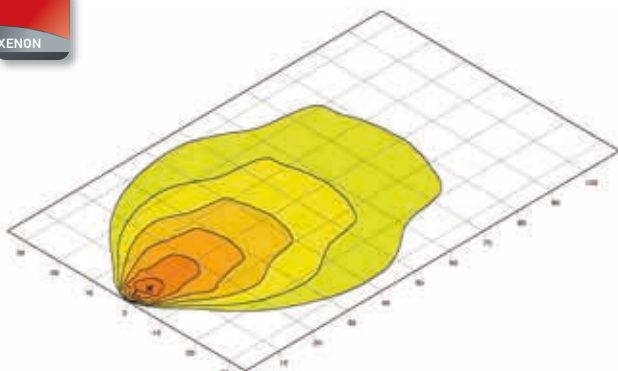
Ultra Beam X-PowerPack | Close-range illumination Page 71
