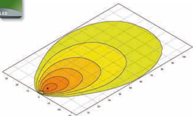
Power Beam 5000 | Close-range illumination Page 52
