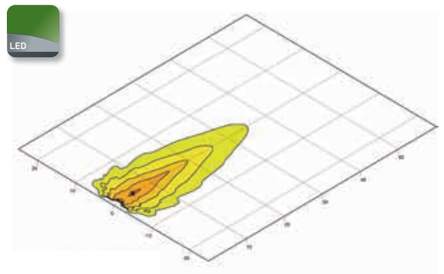
AP 700 LED | Close-range illumination Page 63
